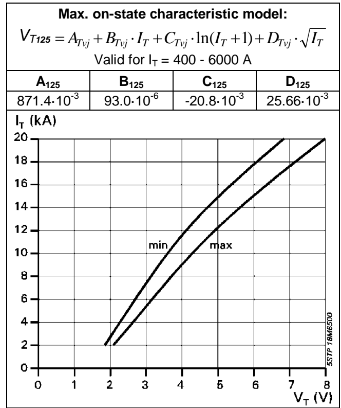
Fig. 3 On-state voltage characteristics, T_{vj\_start} = 125 \text{ }^\circ\text{C} , 10 ms sine half wave
