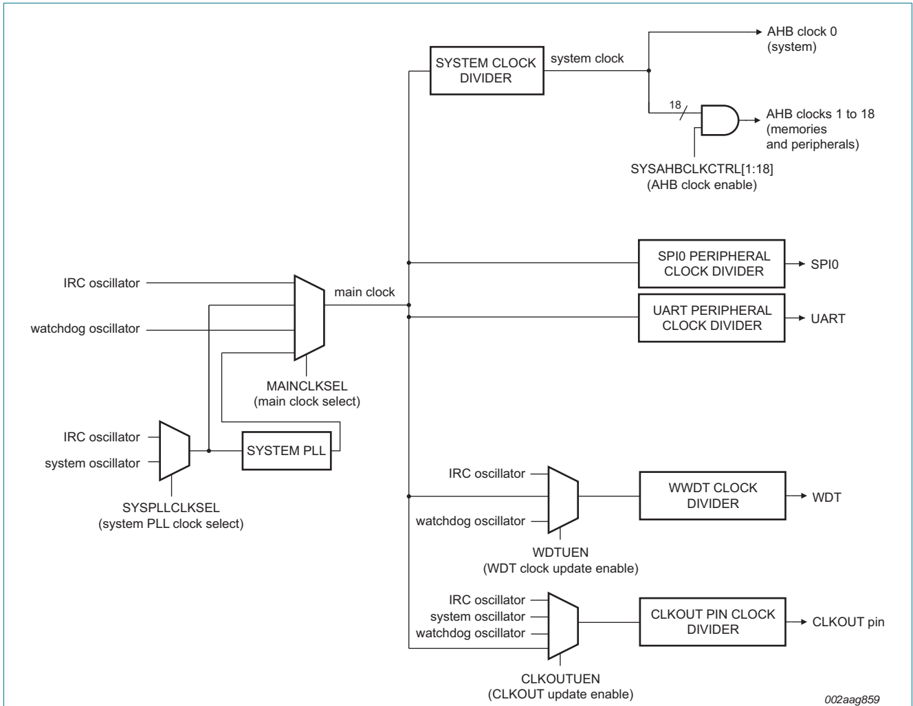
Fig 6. LPC111xLV/LPC11xxLVUK clock generation block diagram
