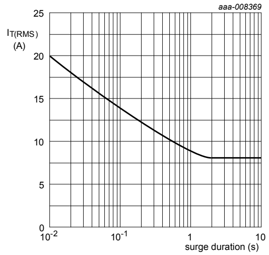
Fig. 3. RMS on-state current as a function of surge duration; maximum values f = 50 \text{ Hz}; T_{mb} = 111 \text{ }^\circ\text{C}
