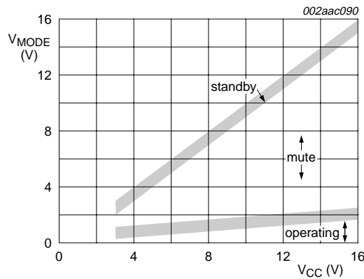
Fig 6. Voltage on pin MODE as a function of supply voltage
