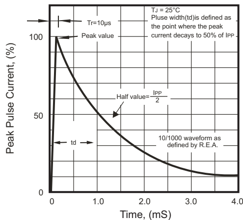
Fig.5 Pulse Waveforem
