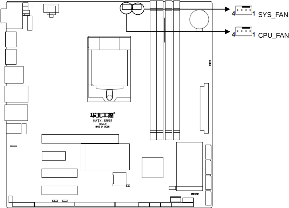
CPU_FAN:
