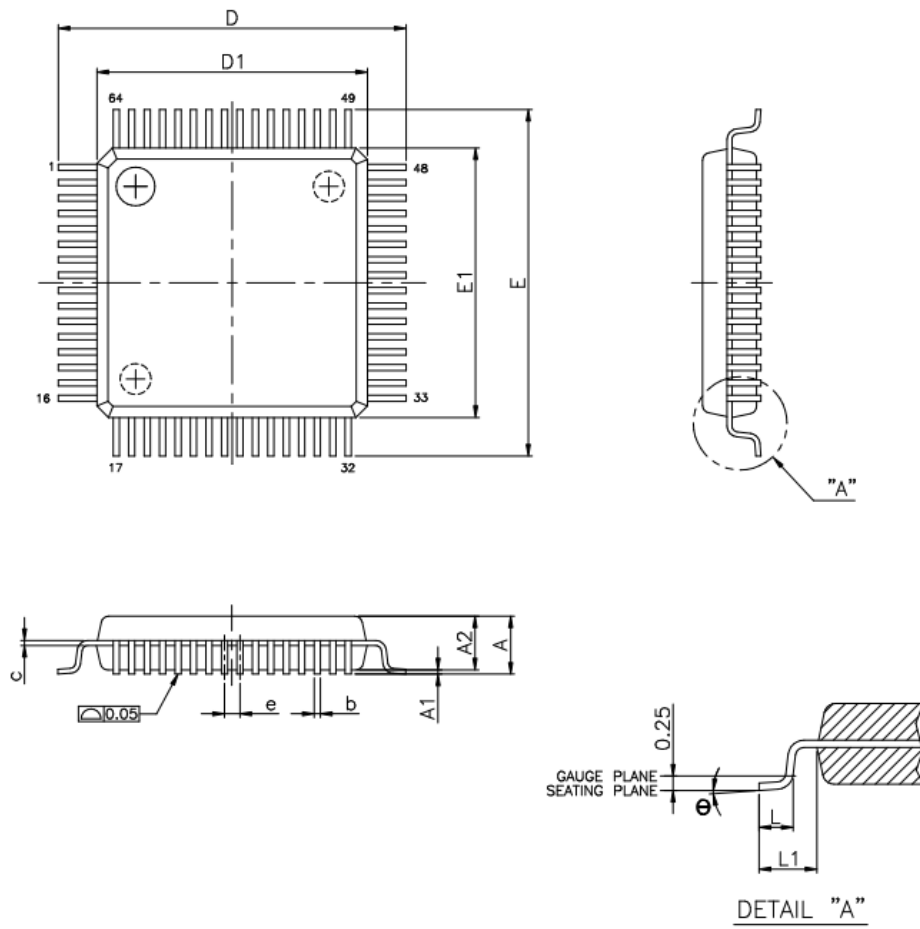
VARIATIONS (ALL DIMENSIONS SHOWN IN MM)
