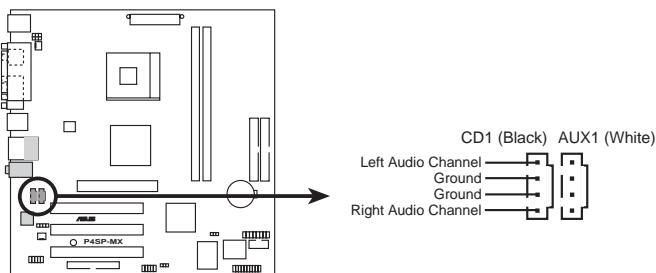
P4SP-MX Internal Audio Connectors
