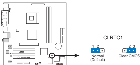
P4SP-MX Clear RTC RAM Setting
