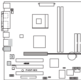
P4SP-MX Accelerated Graphics Port (AGP)
