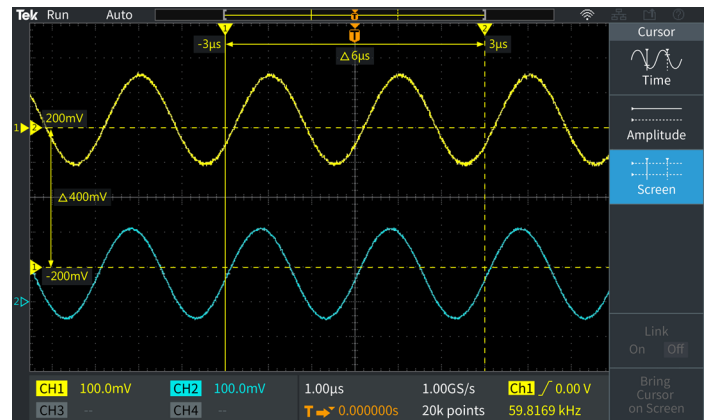
The cursor readouts are presented on the waveform display. Cursors can be used to measure time, amplitude, or both.
