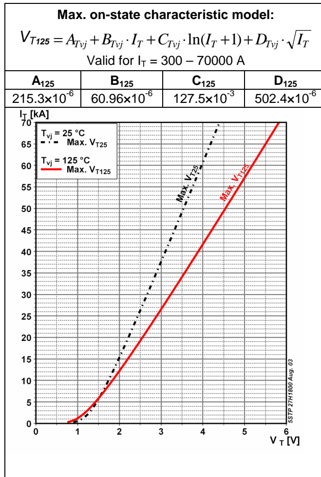
Fig. 3 On-state characteristics, T_{vj} = 125^\circ\text{C} , 10ms half sine
