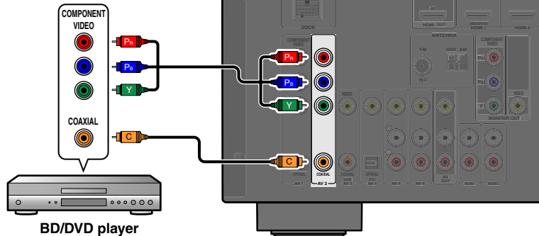
Component video / Audio (Coaxial) output
