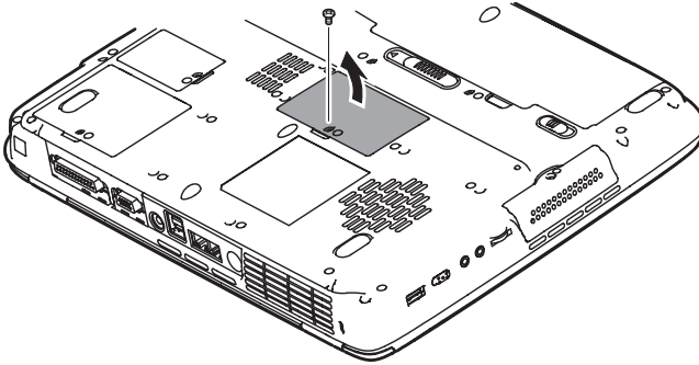
Figure 8-5 Removing the cover
