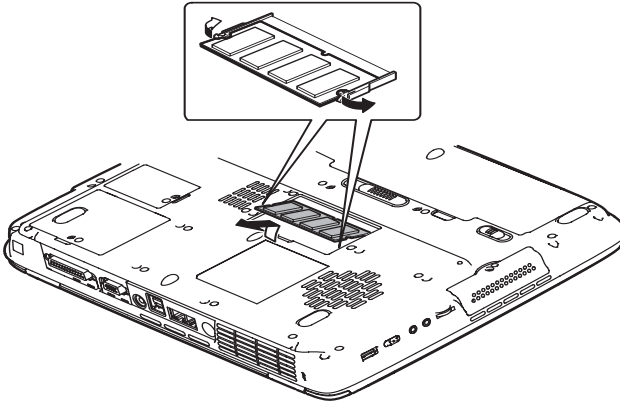
Figure 8-7 Removing the memory module
