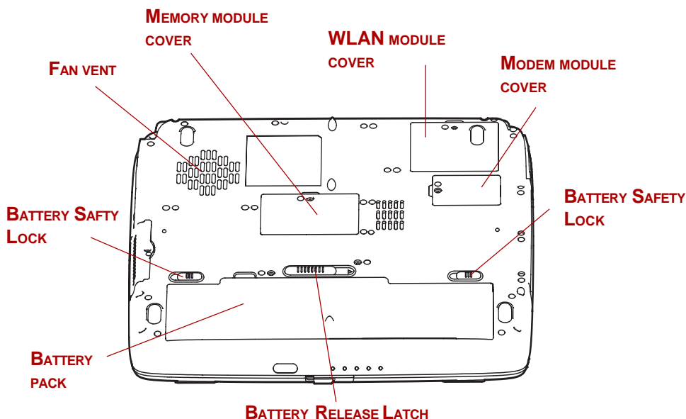
Figure 2-5 The underside of the computer
