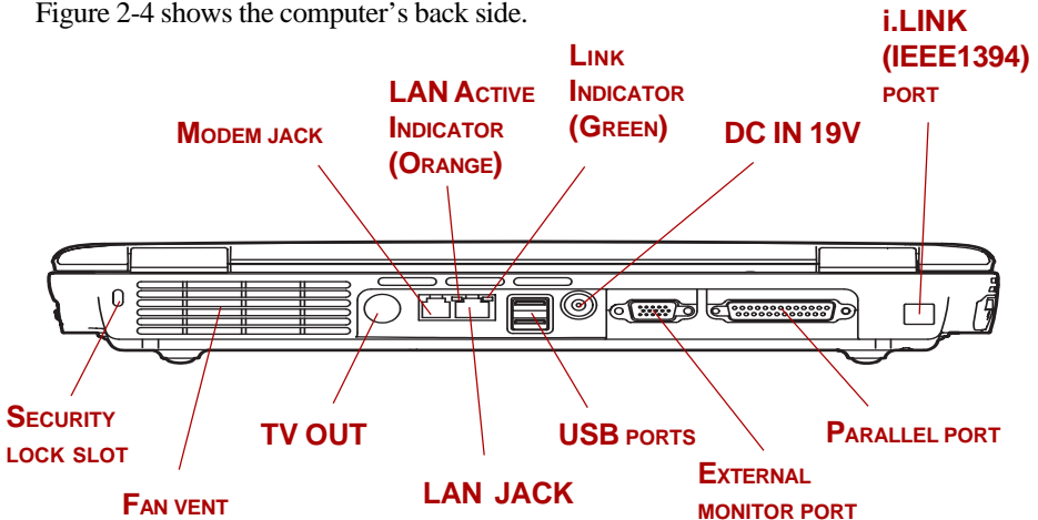
Figure 2-4 The computer's back side
