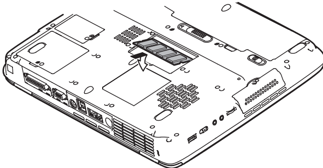
Figure 8-6 Inserting the memory module
