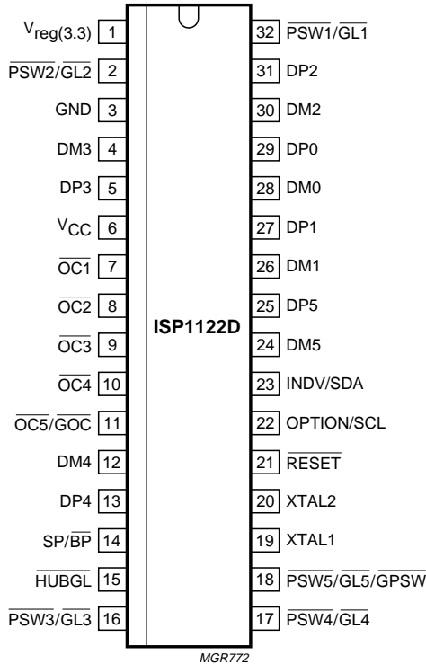
Fig 2. Pin configuration SO32.
