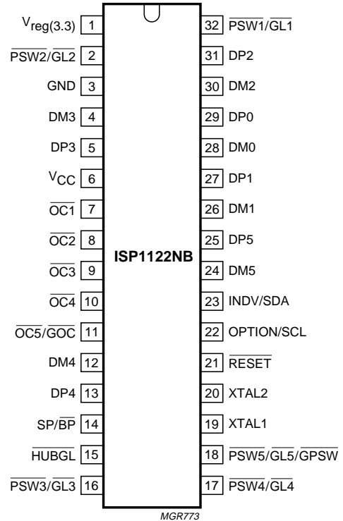
Fig 3. Pin configuration SDIP32.
