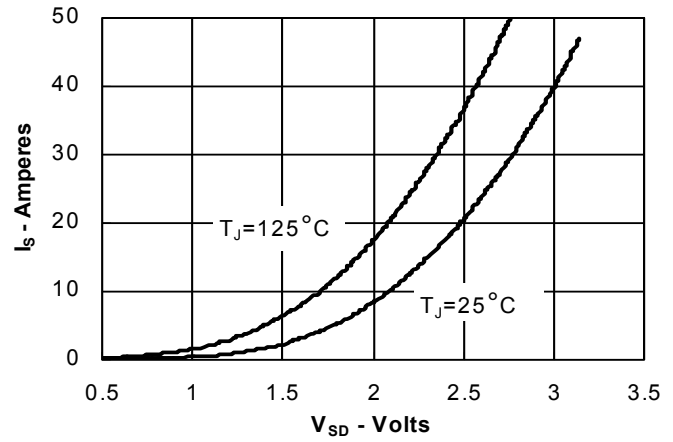
Fig. 8. Source Current vs. Source-To-Drain Voltage
