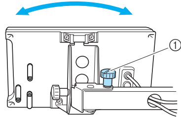
① Thumb screw
