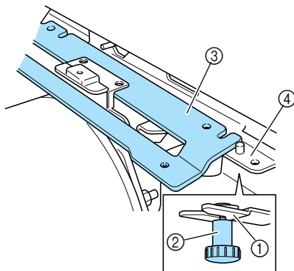
① Notch in the carriage ② Thumb screw of the cap frame driver ③ Mounting plate of the cap frame driver ④ Frame-mounting plate of the carriage
