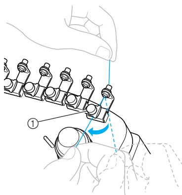
① Upper thread guide
