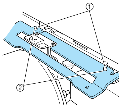
① Pins on the frame-mounting plate of the carriage ② Holes in the mounting plate of the cap frame driver
