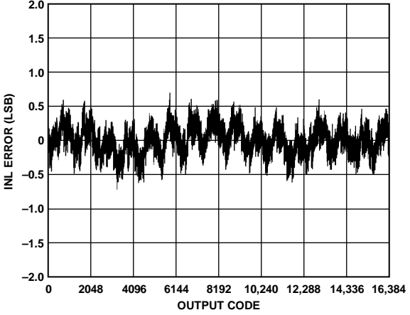
Figure 15. AD9649-80 INL Error with f_{IN} = 9.7 MHz
