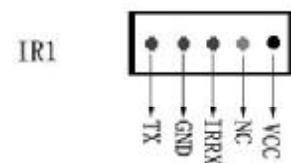
Infrared Module Headers
