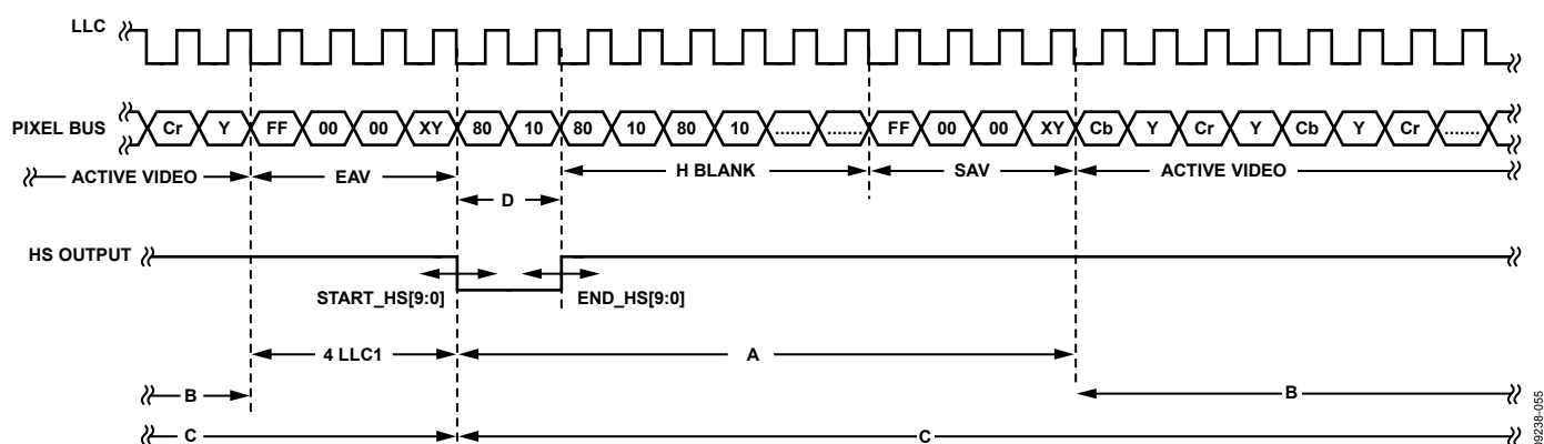
Figure 49. HS Timing
