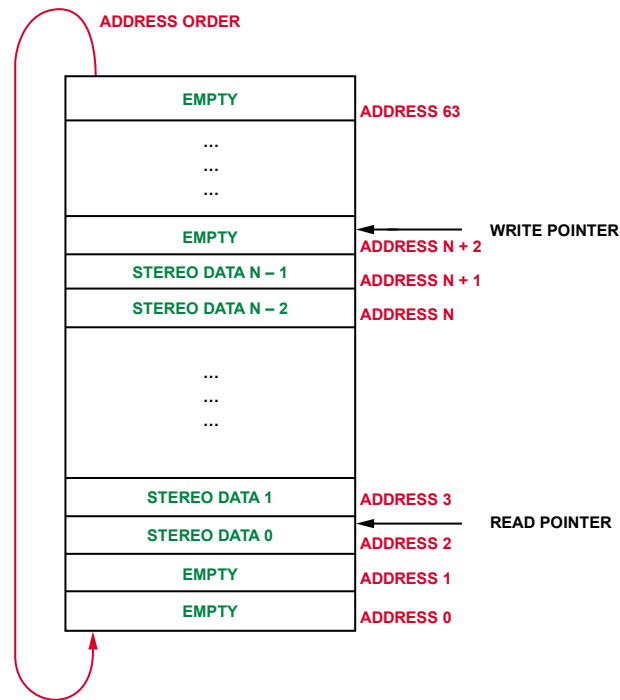
Figure 12. Audio FIFO
