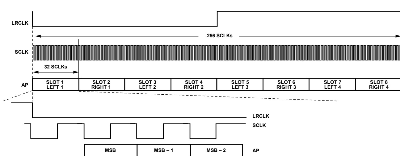
Figure 20. I²S TDM Stream
