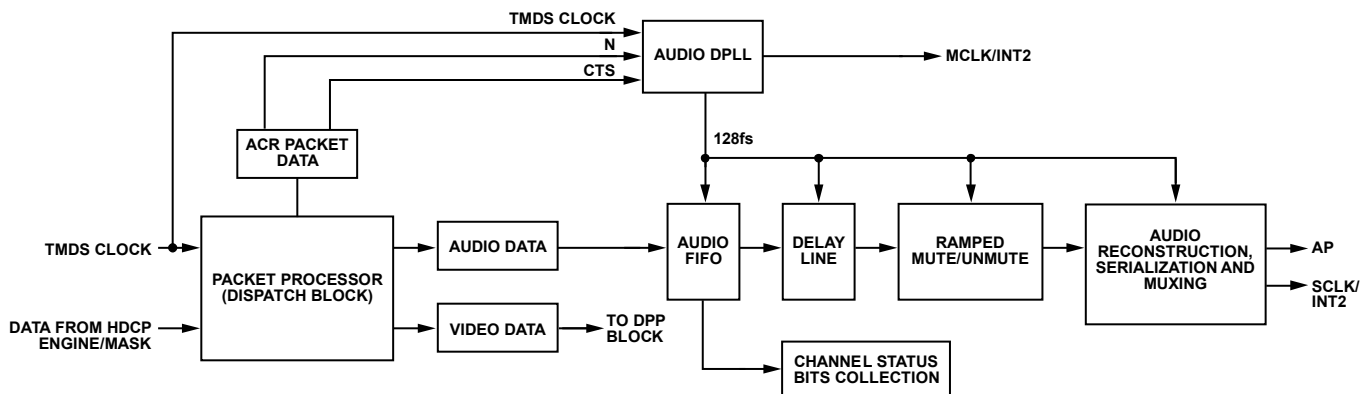
Figure 11. Audio Processor Block Diagram
