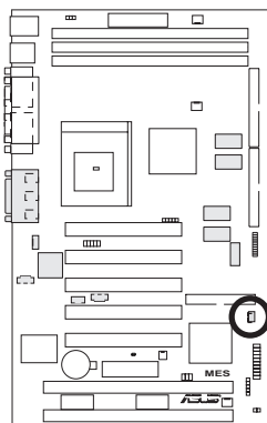
MES Wake-On-LAN Connector
