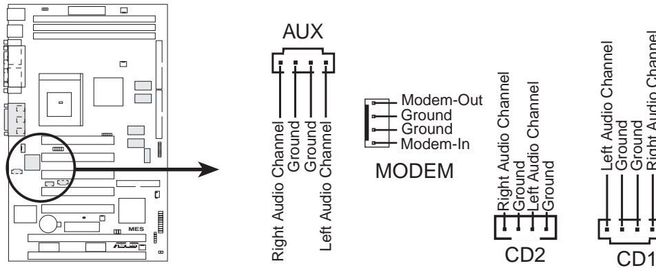
MES Internal Audio Connectors
