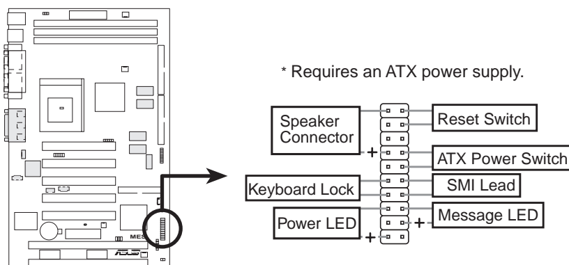
MES System Panel Connectors
