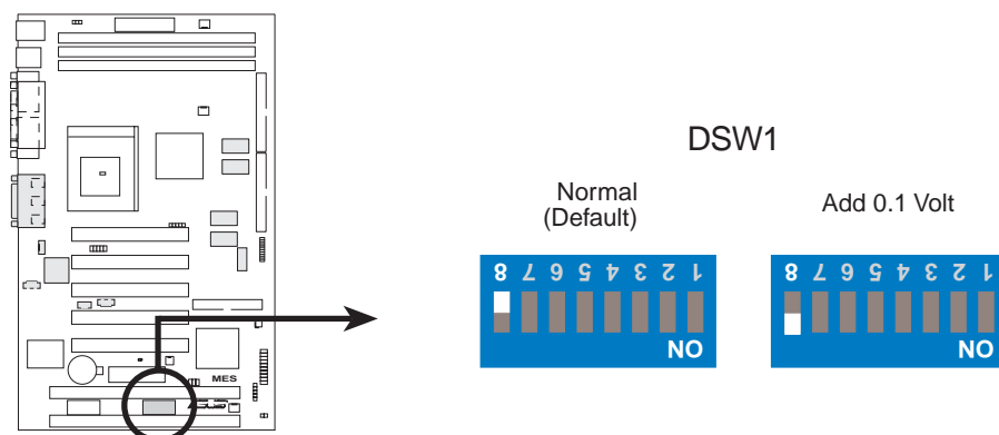
MES CPU Core Voltage (Vcore) Setting
