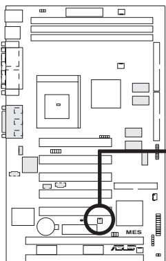
MES Wake-On-Ring Connector
