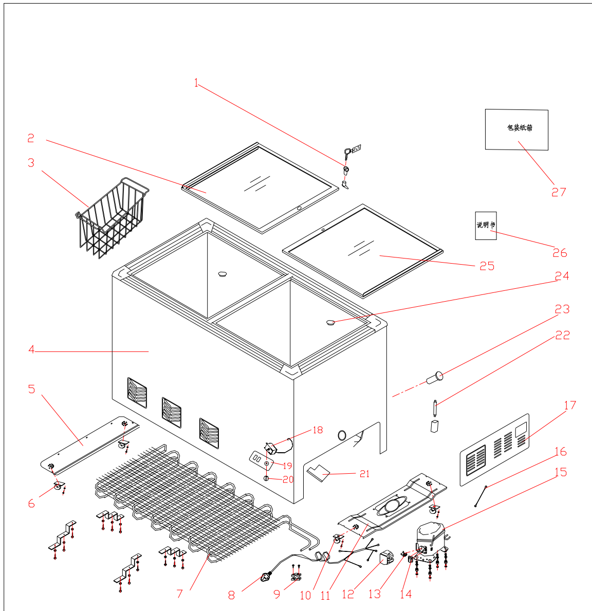
SCD-189GB/209GB/229GB 爆炸图
