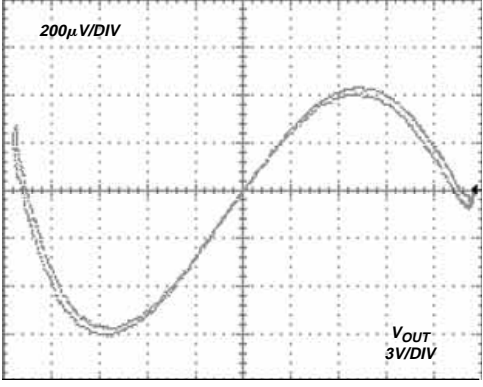
Figure 30. Gain Nonlinearity, V_S = \pm 15 V , G = +5 (7 ppm/DIV)
