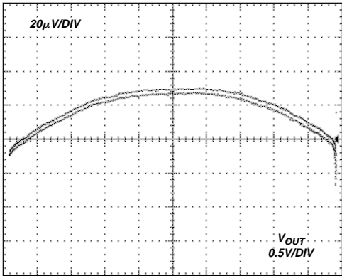
Figure 26. Gain Nonlinearity, V_S = \pm 2.5 V , G = 5 (4 ppm/DIV)
