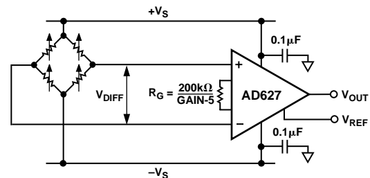
Figure 45. A Classic Bridge Circuit
