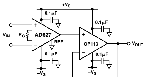
Figure 37. Output Buffering
