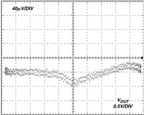
Figure 27. Gain Nonlinearity, V_S = \pm 2.5 V , G = 100 (8 ppm/DIV)
