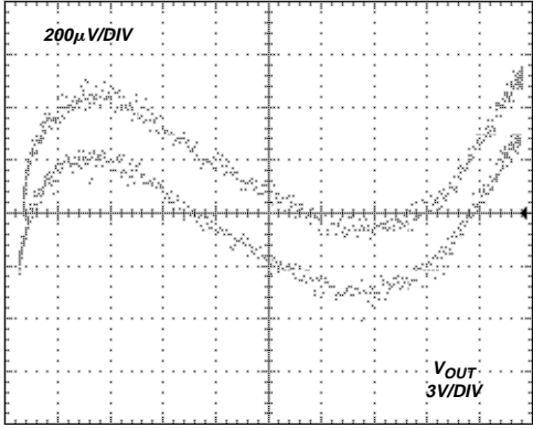
Figure 31. Gain Nonlinearity, V_S = \pm 15 V , G = +100 (7 ppm/DIV)
