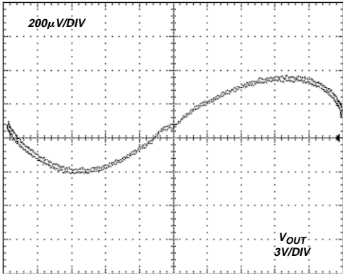
Figure 29. Gain Nonlinearity, V_S = \pm 15 V , G = 100 (7 ppm/DIV)
