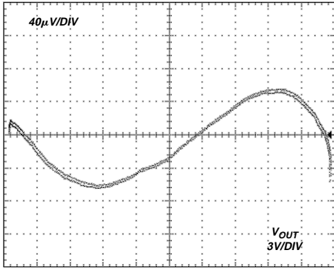
Figure 28. Gain Nonlinearity, V_S = \pm 15 V , G = 5 (1.5 ppm/DIV)
