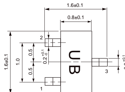
PACKAGE OUTLINE 19
