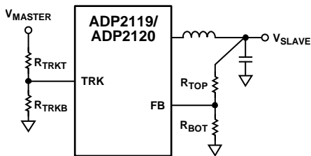
Figure 51. Voltage Tracking
