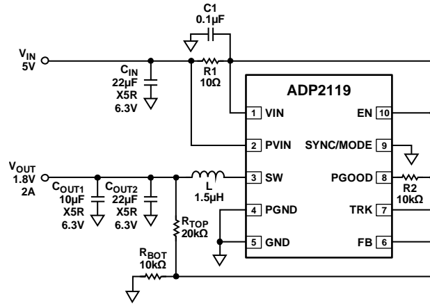
Figure 55. 1.8 V, 2 A, Step-Down Regulator, Enable PFM Mode (ADP2119)
