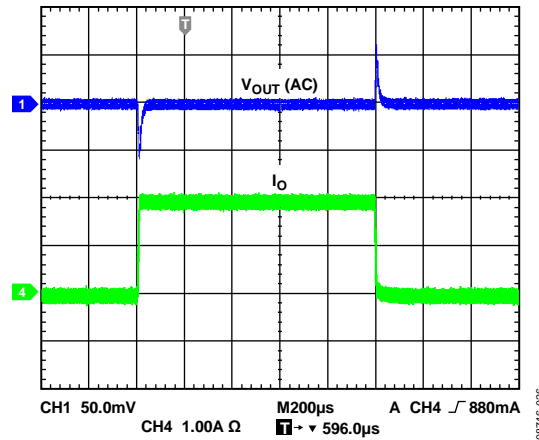
Figure 26. Load Transient (ADP2119, FPWM, V_{IN} = 5V )
