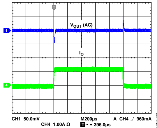
Figure 27. Load Transient (ADP2120, FPWM, V_{IN} = 5V )
