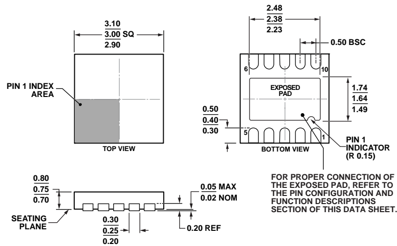
Figure 59. 10-Lead Lead Frame Chip Scale Package [LFCSP_WD] 3 mm × 3 mm Body, Very Very Thin, Dual Lead (CP-10-9) Dimensions shown in millimeters
