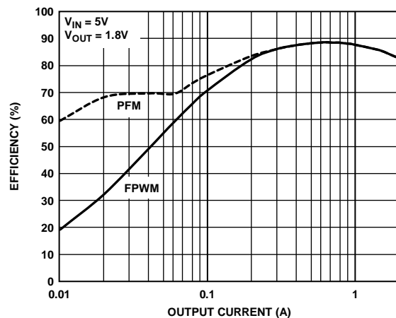
Figure 2. ADP2119 Efficiency vs. Output Current
