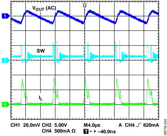
Figure 34. PFM Mode
