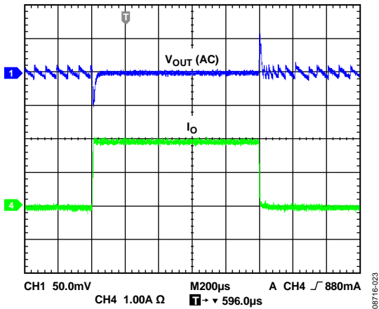
Figure 23. Load Transient (ADP2119, PFM, V_{IN} = 5V )
