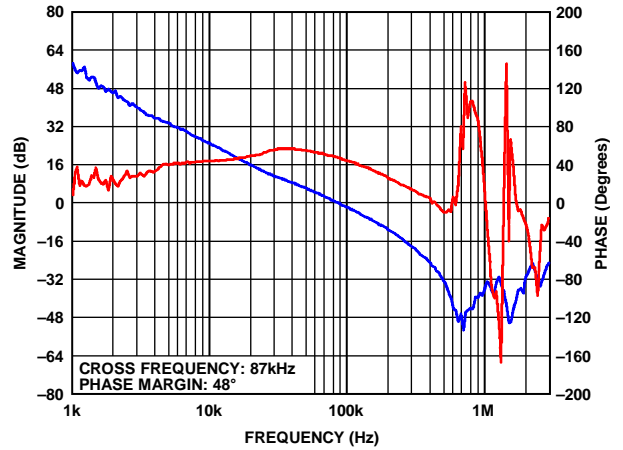
Figure 43. ADP2120 Bode Plot at V_{IN} = 5\text{ V} , V_{OUT} = 1.0\text{ V} , I_O = 1.25\text{ A} , L = 1.5\ \mu\text{H} , C_{OUT} = 22\ \mu\text{F} + 10\ \mu\text{F}
