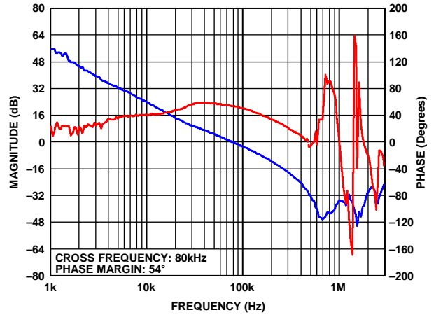
Figure 44. ADP2120 Bode Plot at V_{IN} = 5\text{ V} , V_{OUT} = 1.2\text{ V} , I_O = 1.25\text{ A} , L = 1.5\ \mu\text{H} , C_{OUT} = 22\ \mu\text{F} + 10\ \mu\text{F}
