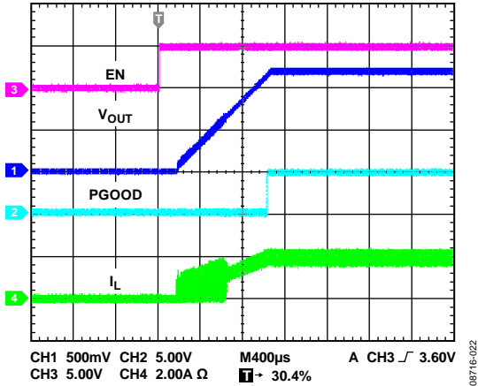
Figure 22. Soft Start with Full Load (ADP2119, V_{IN} = 5V )
