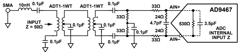
Figure 51. Differential Transformer-Coupled Configuration for Baseband Applications up to 150 MHz
