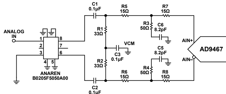
Figure 53. Wideband Balun-Coupled Configuration for IF Applications Up Greater Than 100 MHz
