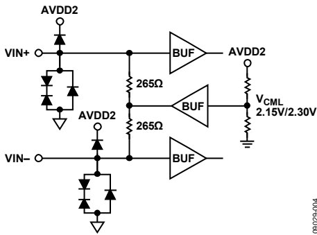
Figure 4. Equivalent Analog Input Circuit
