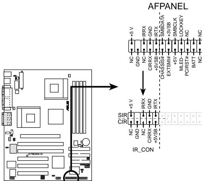
A7M266-D Front Panel Connector
