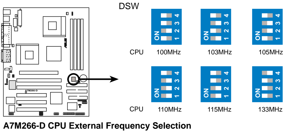
Frequency Table
