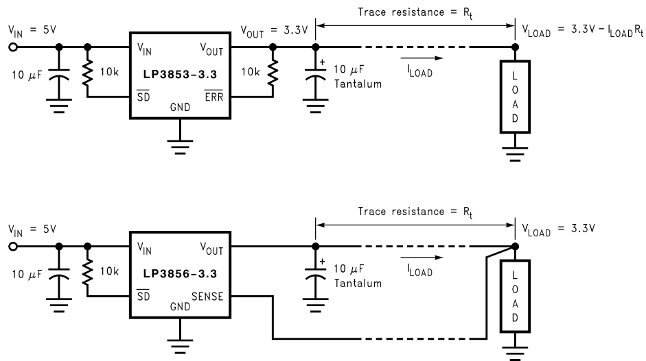
FIGURE 4. Improving remote load regulation using LP3856
