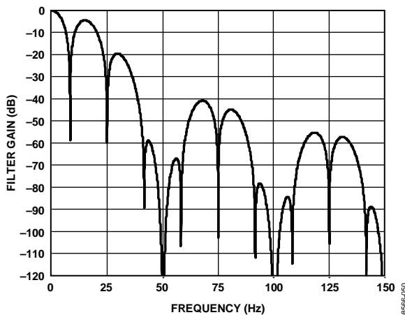
Figure 51. Sinc 3 Filter Response ( FS[9:0] = 96 , Chop Enabled)
