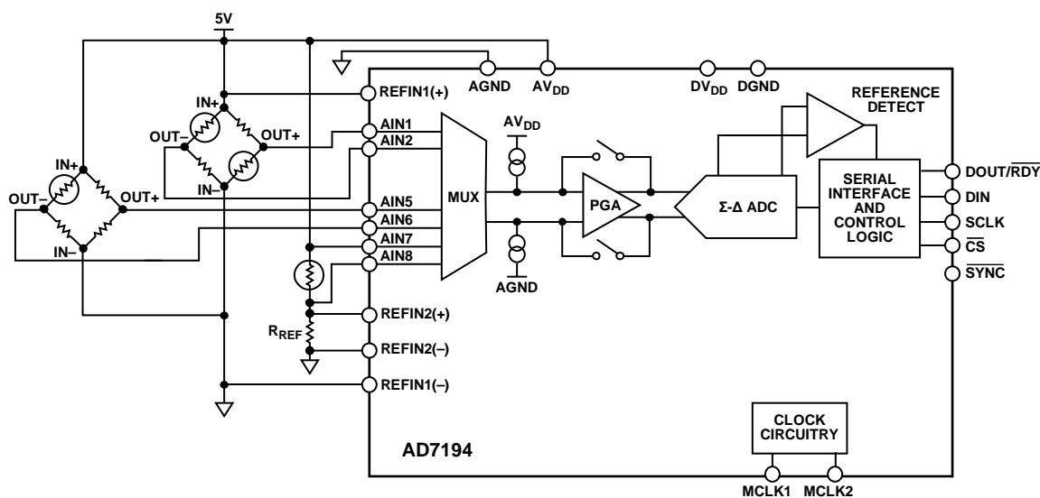
Figure 67. Typical Application (Flowmeter)
