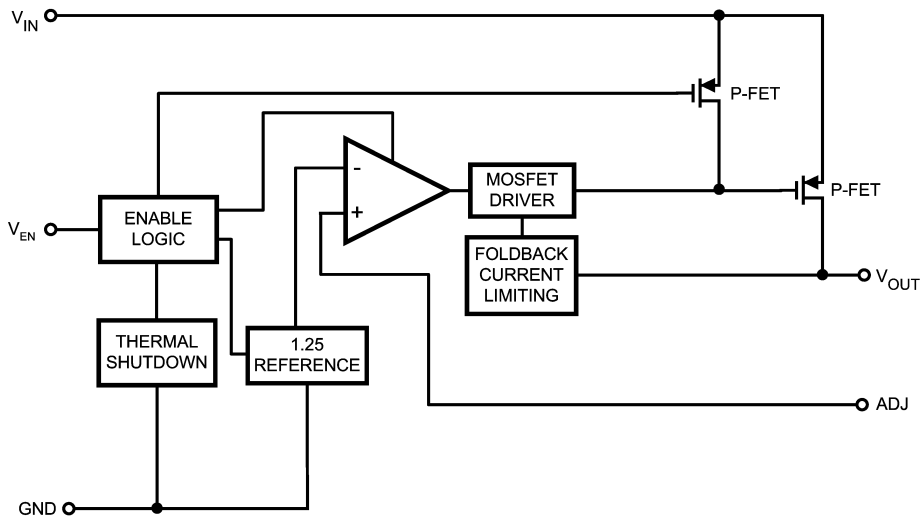
FIGURE 2. LP38693-ADJ Functional Diagram (SOT-223, LLP)
