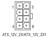
ATX_12V_2X/ATX_12V_2X1
