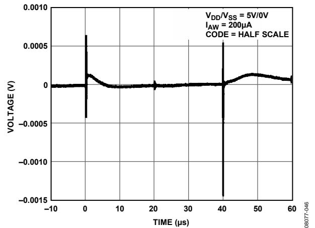
Figure 35. Digital Feedthrough
