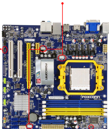
CPU_FAN/SYS_FAN/ NB_FAN
