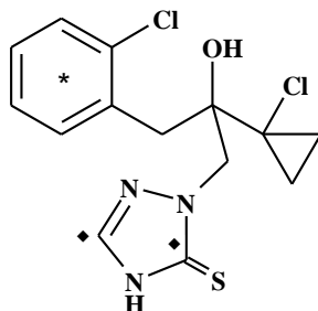
phenyl-UL- ^{14}\text{C} - and 3,5-triazole- ^{14}\text{C} -prothioconazole
