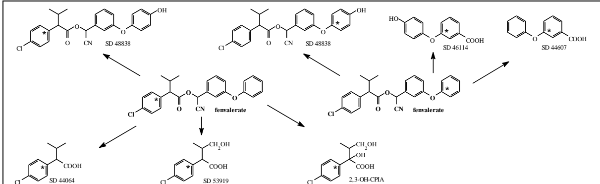
Figure 2. Livestock metabolism of fenvalerate 14 C labelled in the chlorophenyl ring or the phenoxyphenyl ring. The asterisk * indicates the position of the label.
