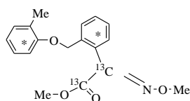
Krezoxim-methyl
