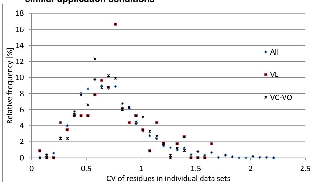
Figure 2. Relative frequency of CV values of data sets of leafy vegetables, including Brassica leafy vegetables (VL), fruiting vegetables, other than cucurbits (VO) fruiting vegetables, cucurbits (VC) commodity groups and all data (All).
