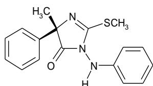
Fenamidone
