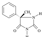
RPA412636
