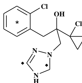
phenyl-UL- ^{14}\text{C} - and 3,5-triazole- ^{14}\text{C} -desthio prothioconazole
