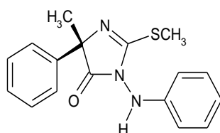
Fenamidone
